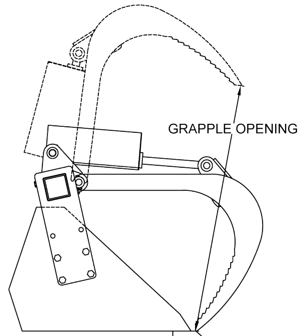
(Typical installation of Model 222 Contractor Add-A-Grapple)
